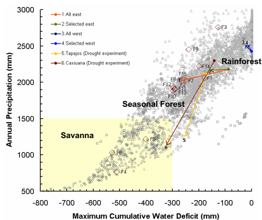
Fig. 3. Drought experiments and field observations of forest fire in the context of the mean of GCM projections in change of rainfall regime in E. and W. Amazonia. For the GCMs, the arrow base indicates late 20th-century rainfall regime whereas the arrow tip indicates late 21st-century rainfall regime. For the drought experiments, the arrow base indicates control rainfall regime whereas the arrow tip indicates the estimated rainfall regime. Diamonds indicate field studies of flammable forests (see Table S3), with rainfall regimes derived from TRMM (1998–2006). Our suggested savanna zone is shaded (MCWD < -300 mm, AP < 1500 mm).
