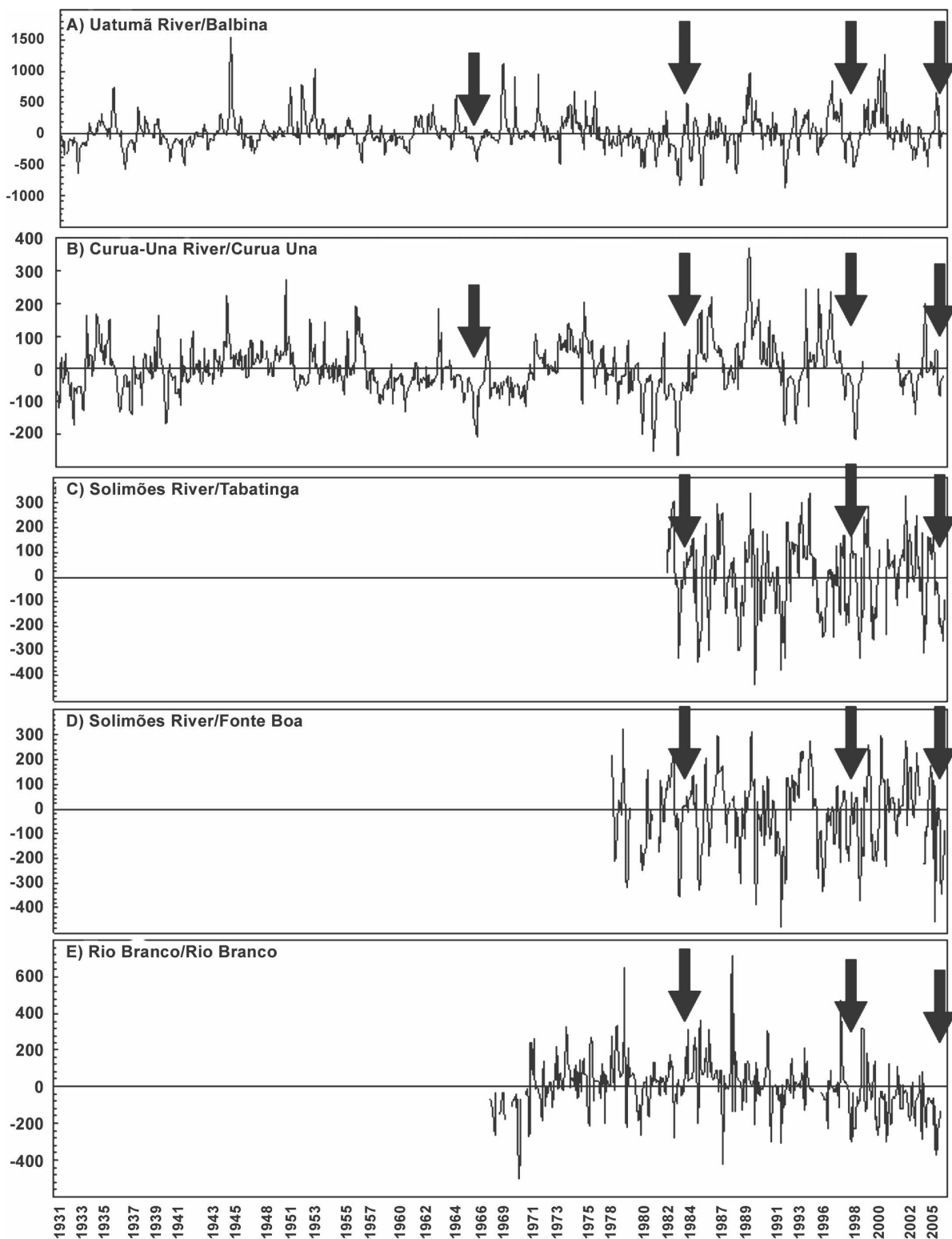
FIG. 5. (a)–(e) Monthly river levels/streamflow anomalies from 1931 to 2005 for the Uatumã River in Balbina and Curua Una River in Curua Una, from Solimões River in Tabatinga (1982–2005), and in Fonte Boa and Acre River in Rio Branco (1971–2005). Arrows indicate dry years 1964, 1983, 1998, and 2005. (Source of data: ANA.)
