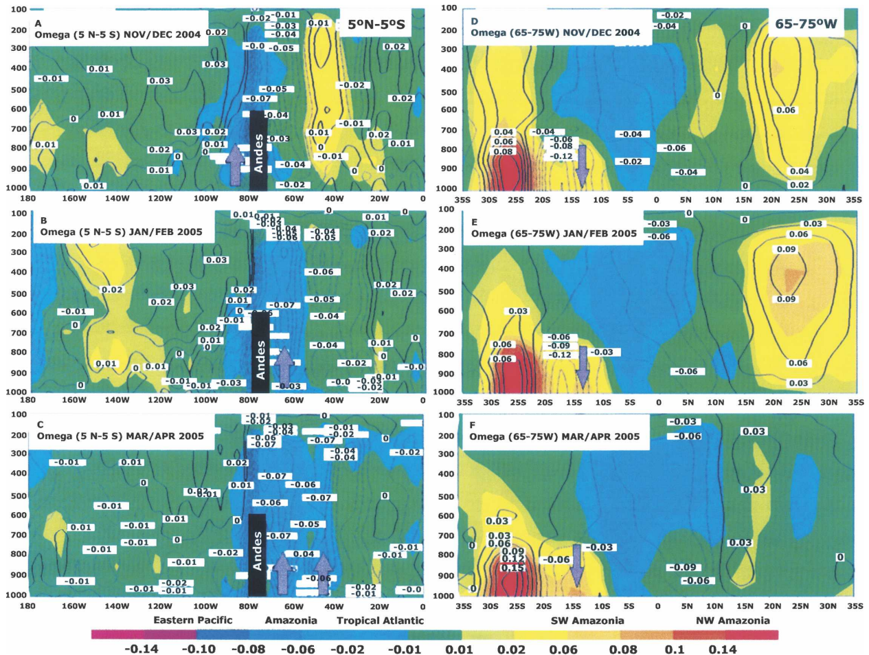
FIG. 10. Vertical cross sections of vertical velocity anomalies during November–December 2004, January–February 2005, and March–April 2005. (left) A zonal equatorial cross section along 5^{\circ}\text{N} – 5^{\circ}\text{S} ; (right) a meridional cross section along 65^{\circ} – 75^{\circ}\text{W} . Lines represent the observed values of vertical motion ( \text{Pa s}^{-1} ), and anomalies (from the 1979–2005 mean) are in color with the color scale bar at the bottom. The vertical black box represents the approximate location of the Andes.
