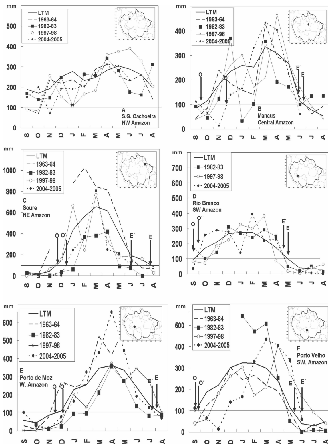
FIG. 3. Rainfall during various drought years (1963–64, 1982–83, 1997–98, and 2004–05) in stations in various sectors of Amazonia (source of data: ANA, CTA). The hydrological year is September–August. The mean is from the 1961–90 LTM. O/E represents the climatic onset/end of the rainy season, and O'/E' represents the onset/end of the rainy season during 2004–05. The threshold value of 100 \text{ mm month}^{-1} is shown as indicator of the dry season (Sombroek 2001).
