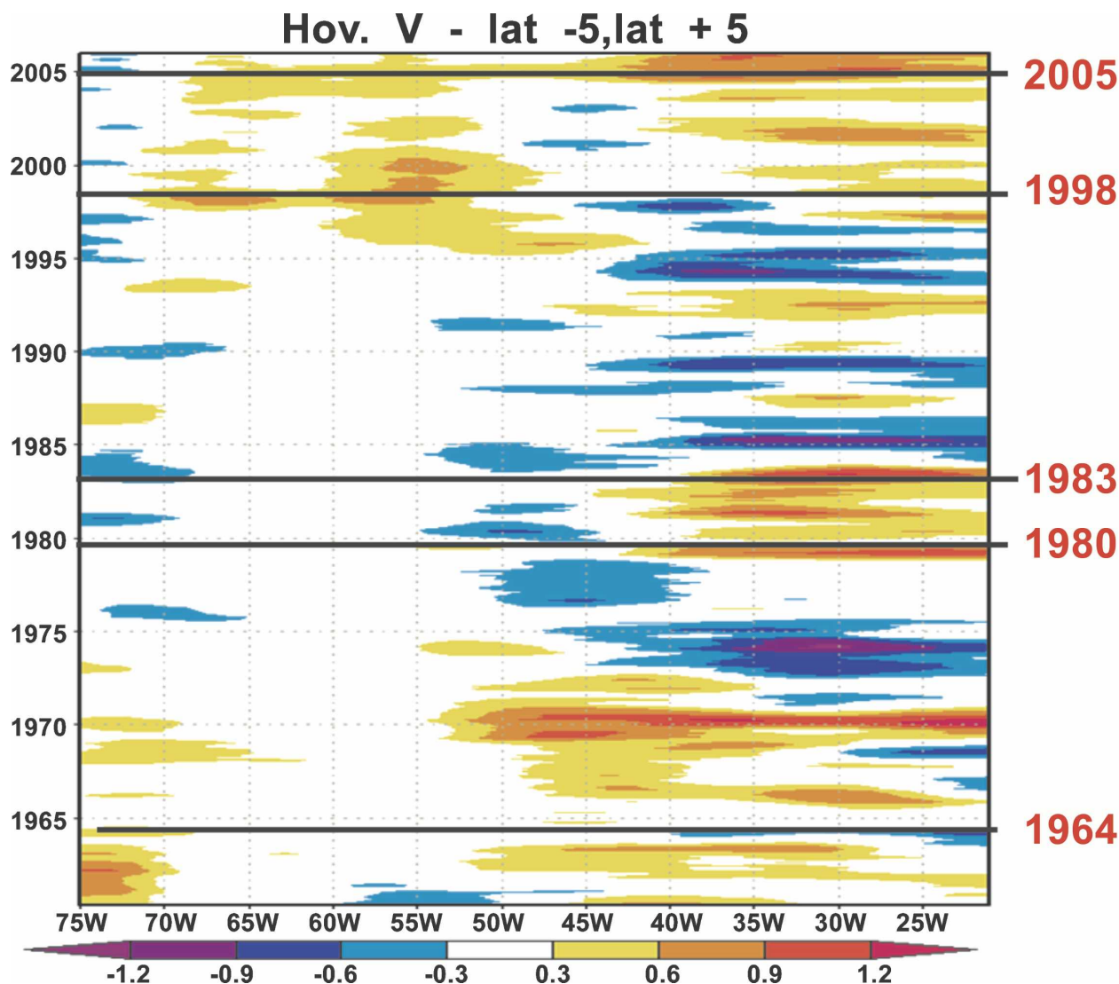
FIG. 9. Hovmöller diagram of meridional wind anomaly between 75° and 20°W, for the equatorial band of 5°N–5°S. Positive/negative values indicate southerly/northerly wind anomalies, with respect to the 1979–2005 mean.
