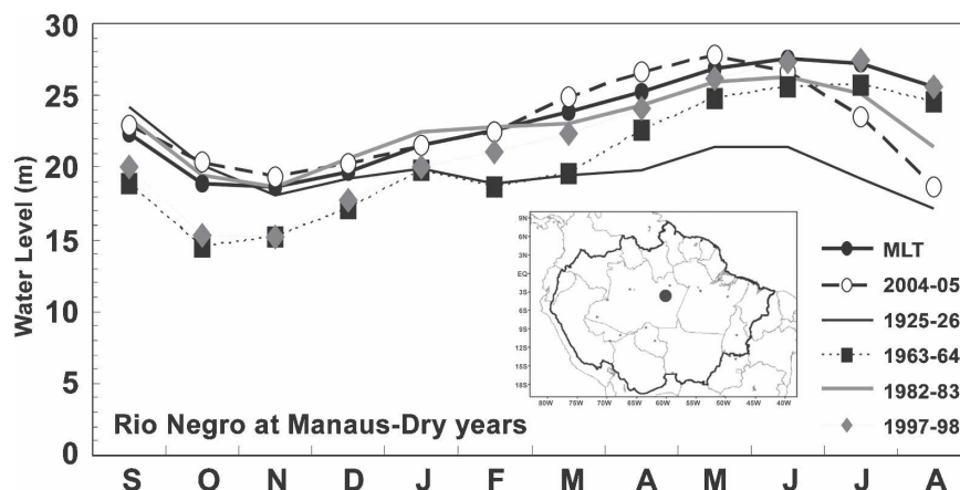
FIG. 13. Rio Negro water levels (m) in Manaus station during selected dry years. The long-term mean is 1903–2000. Location of Manaus is shown by a dot in the inset map.
