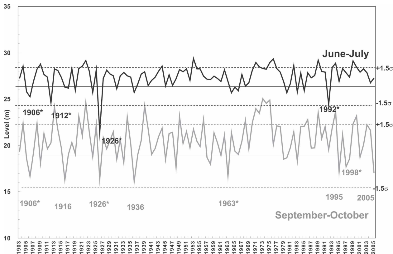
FIG. 2. Rio Negro water levels at Manaus (m) in the Manaus station, Brazil, during the peak water-level season in June–July (black lines) and the low water-level season in September–October (gray lines). Full/thin broken lines represent the mean \pm 1.5\sigma . The number indicates years where the levels reached values lower than 1.5\sigma . Asterisks depict El Niño years. (Source of river data: ANA, PORTOBRAS.)
