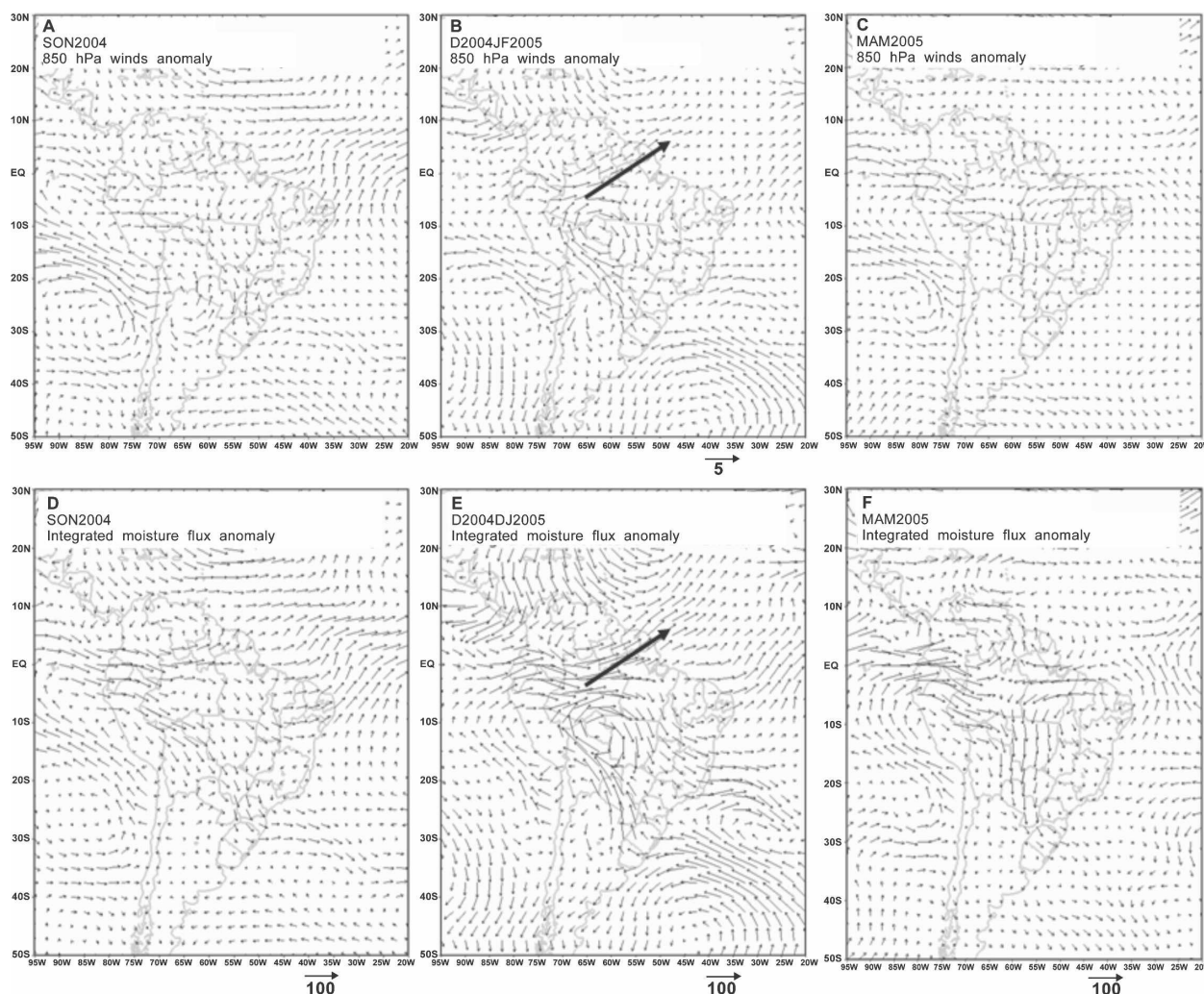
FIG. 8. Low-level circulation and integrated moisture flux anomalies in South America for SON 2004, DJF 2004–05, and MAM 2005. (a)–(c) The circulation anomalies and (d)–(f) the integrated moisture flux anomalies from the 1979–2005 mean. Vector with the scale of the wind/flux is shown at the bottom of each panel.
