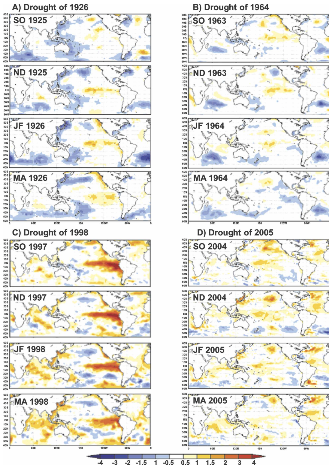
FIG. 12. (a)–(d) SST anomalies ( ^{\circ}\text{C} ) during SO, ND, JF, and MA during some years with drought conditions in Amazonia (1925–26, 1963–64, 1997–98, and 2004–05). SST anomalies are in relation to the 1961–90 baseline period. Color scale is shown at the bottom of the figure.
