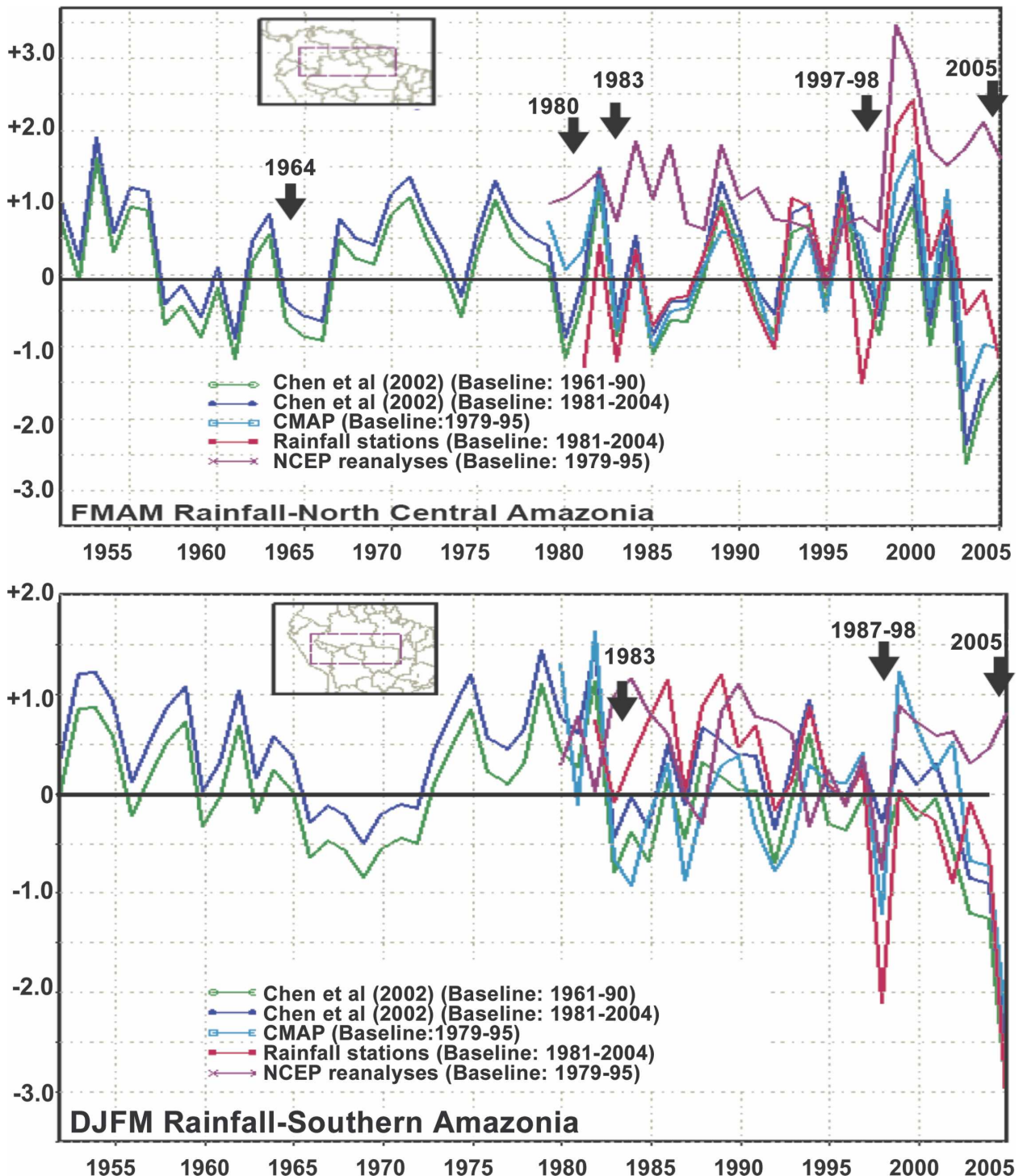
FIG. 4. Time series of rainfall indices for (a) northern Amazonia (FMAM) and (b) southern Amazonia (DJFM) from 1950 to 2005. These seasons correspond to the peak of the rainy season in those sections of the Amazon basin. Rainfall datasets are from Chen et al. (2002), CMAP (Xie and Arkin 1997), and an index derived from rainfall stations. Anomalies ( \text{mm day}^{-1} ) are derived using different baseline periods. Arrows indicate major drought events for this period.
